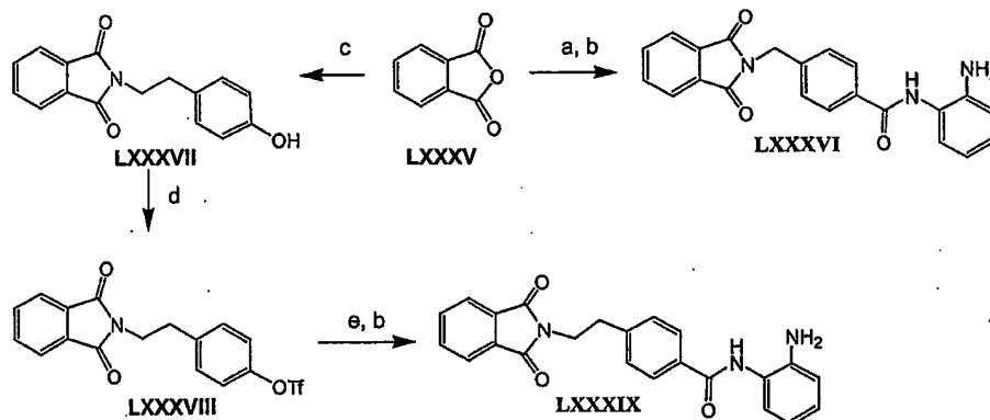
Scheme 18
